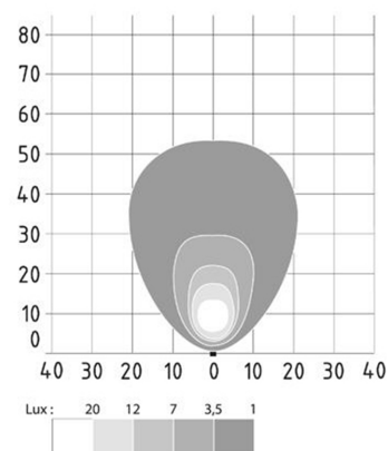
FLOOD ASYMMETRICAL
